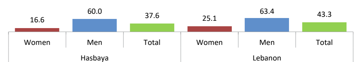
Figure 23: Employment-to-population ratio (%)
